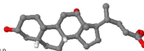
Deoxycholic acid (3D)
